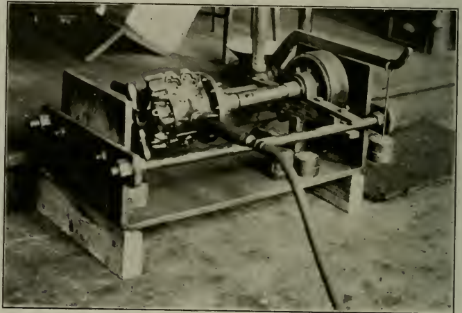
PRONG BRAKE FOR TESTING AIR MOTORS
